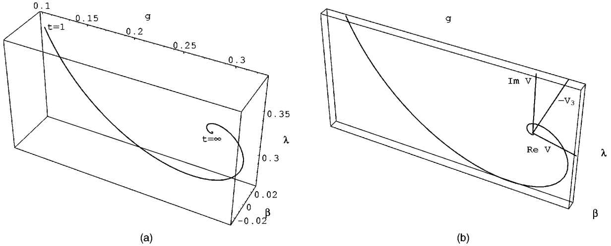
FIG. 5. Trajectory of the linearized flow equation obtained from the R^2 truncation for 1 \leq t = \ln(k/k_0) < \infty . In (b) we depict the eigendirections and the “box” to which the trajectory is confined.
