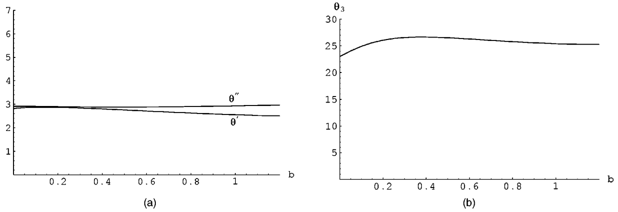
FIG. 7. (a) \theta' = \text{Re}\theta_1 and \theta'' = \text{Im}\theta_1 , and (b) \theta_3 as functions of b , using the family of shape functions with compact support.
